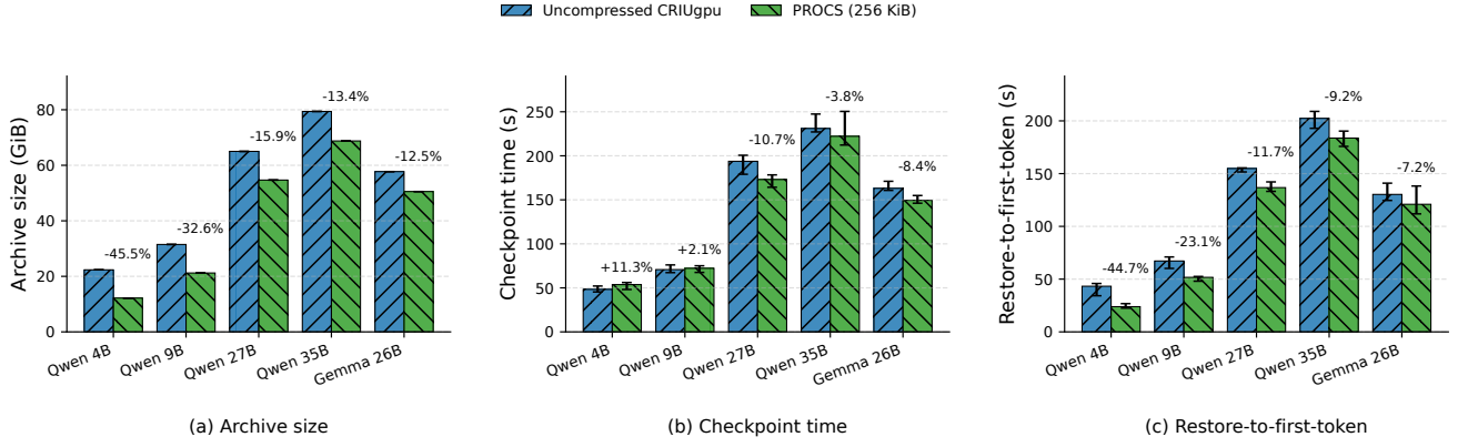
Fig. 4. End-to-end comparison between uncompressed CRIUgpu and PROCS with 256 KiB blocks across five SGLang inference models. Both configurations use one decompression thread. Bars show medians over five repetitions, error bars show deterministic bootstrap 95% confidence intervals, and annotations report changes relative to uncompressed CRIUgpu.
