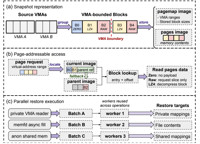
Fig. 3. PROCS separates persistent representation, page-addressable access, and restore execution. (a) Pages are grouped into VMA-bounded blocks stored in zero, LZ4, or raw form. (b) Block-aware readers translate page-range requests, including parent-image lookups, into bounded batches. (c) Reader-owned worker pools execute reconstruction jobs under a shared restore-wide decompression budget. Blocks determine storage, batches bound I/O and buffering, and jobs expose parallel reconstruction.
