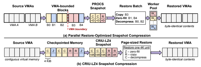
Fig. 1. Comparison of memory snapshot formats and restore paths. (a) PROCS groups pages into VMA-bounded blocks, combines block data into restore batches, and restores them in parallel using worker pools. (b) CRIU-LZ4 compresses and restores each 4 KiB page independently. Labels C, R, and Z denote compressed , raw , and zero representations, respectively.
