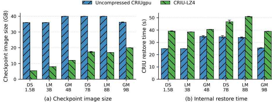
Fig. 2. Comparison between CRIU-LZ4 and uncompressed CRIUgpu for six vLLM [8] inference workloads on an NVIDIA A100 (SXM4 40GB): (a) checkpoint size and (b) restore latency. Compared to uncompressed CRIUgpu snapshots, CRIU-LZ4 reduces checkpoint image size by \approx 45\text{--}85\% but increases restore latency with 16.3\text{--}57.4\% . Bars show means, and error bars show standard errors ( n = 3 or 5 per model) where checkpoint images resided in memory-backed filesystem. Model labels DS, LM, and GM denote DeepSeek, Llama, and Gemma, respectively with suffix indicating a parameter count in billions.
