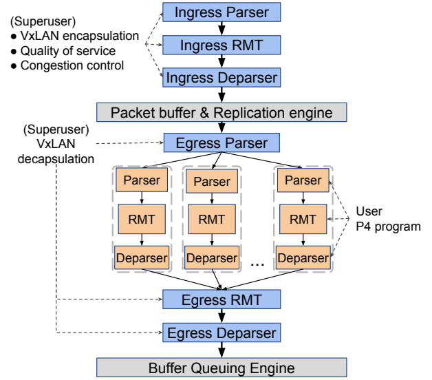
Figure 2: Block diagram of the MTPSA P4 architecture.
