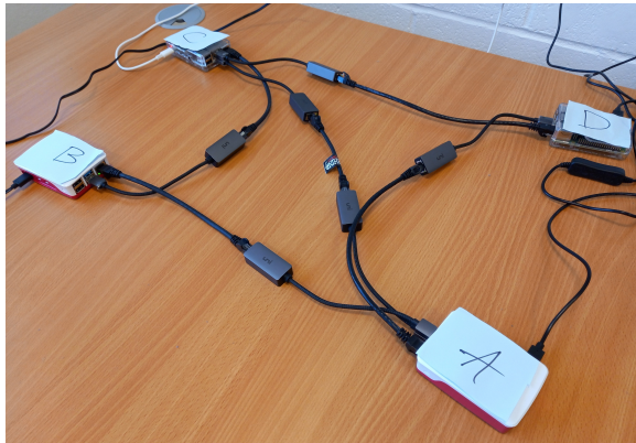
Figure 3: P4Pi Interoperability Setup.
